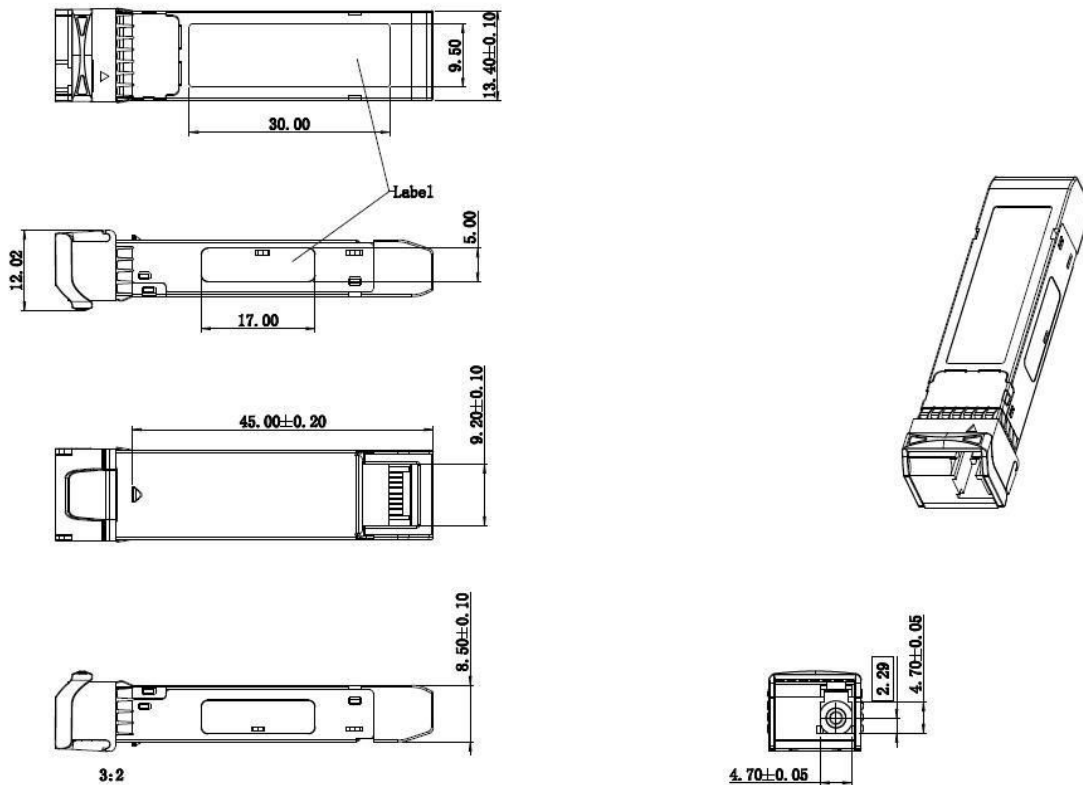
Figure 3. Mechanical Specifications
